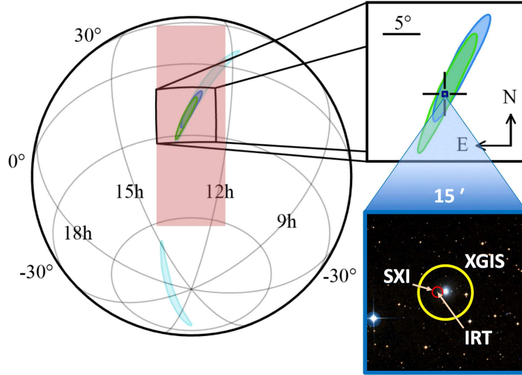
Fig. 1. The plot shows the THESEUS/SXI field of view ( \sim 110 \times 30 \text{ deg}^2 , pink rectangle) superimposed on the probability skymap of GW 170817 obtained with the two Advanced LIGO only (cyan) and with the addition of Advanced Virgo (green) (Abbott et al. 2017c). THESEUS not only will cover a large fraction of the skymap (even those obtained with only two GW-detectors, e.g. cyan area), but will also localize the counterpart with uncertainty of the order of 5 arcmin with the XGIS and to less than 1 arcmin with SXI. The THESEUS location accuracy of GW events produced by NS-NS mergers can be as good as 1 arcsec in case of detection of the kilonova emission by the IRT. By the end of the 2020s, if ET will be a single detector, almost no directional information will be available for GW sources ( > 1000 \text{ deg}^2 for BNS at z > 0.3 , Zhao & Wen e.g. 2017), and a GRB-localising satellite will be essential to discover EM counterparts.
